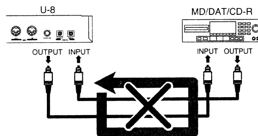
Example of a Digital Loop Connection
