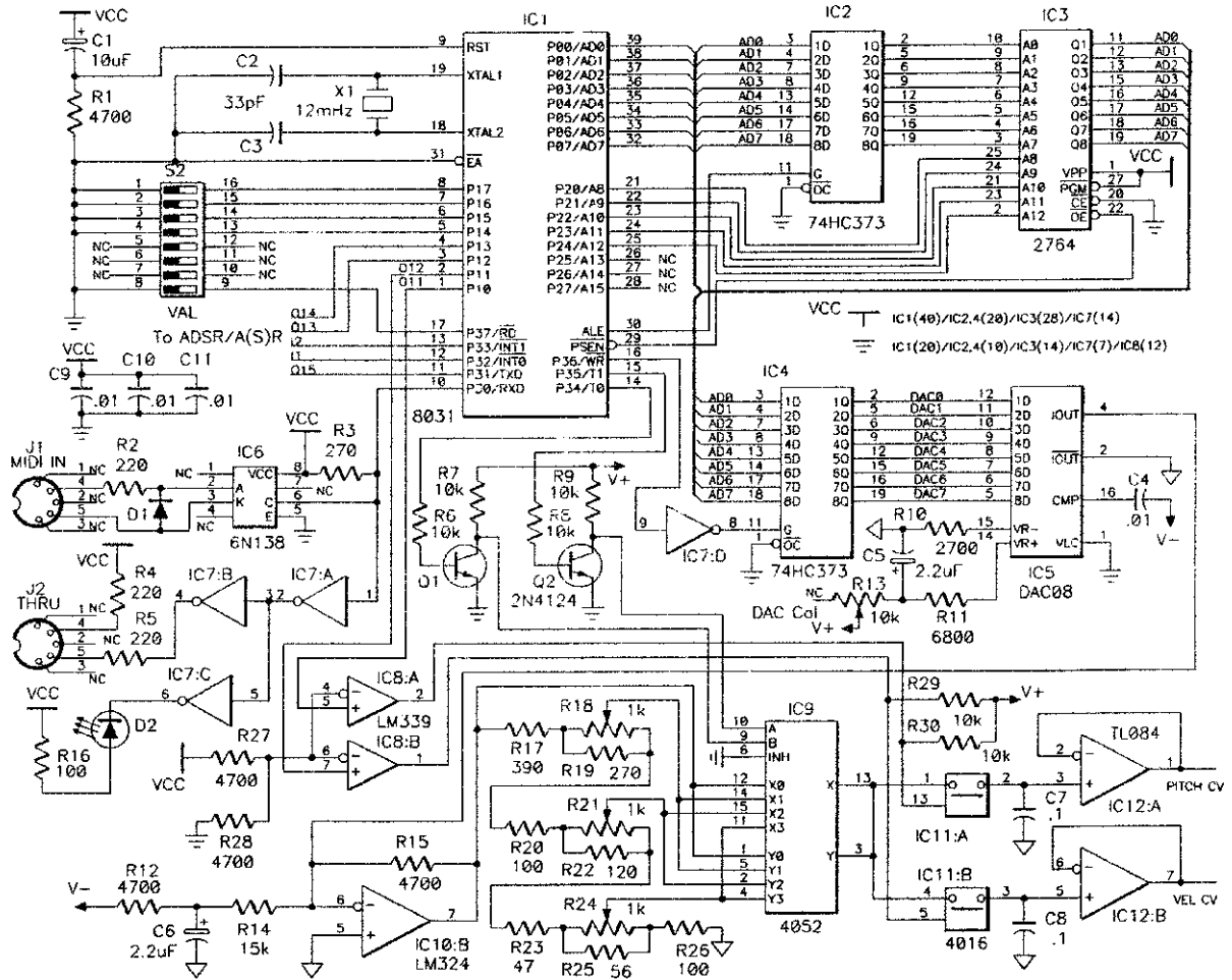
Fig 5a. An 8031 uProcessor provides the computing horsepower needed to decode MIDI and keep Control Voltages straight. Equally tempered Control Voltages are provided by the combination of the DAC and Octave Range switching.
