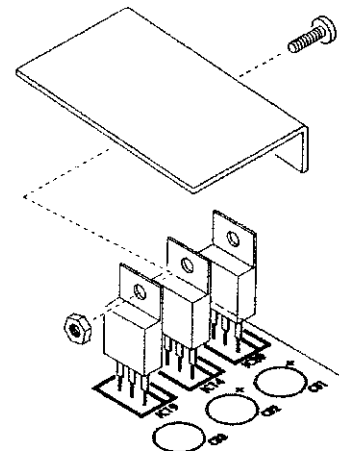
Heat dissipating fin attaches to IC19.
