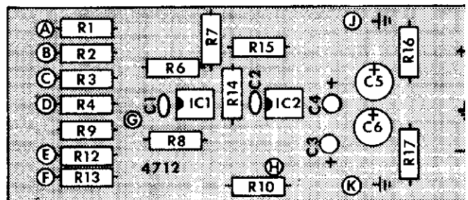
Figure 1 Parts Placement
