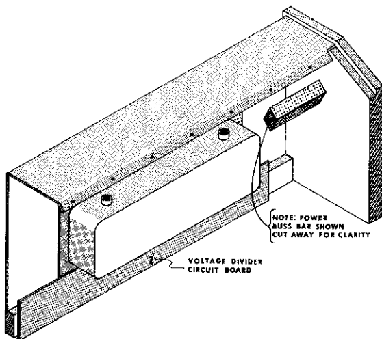
Figure 5 - Mounting the Reverb Spring
