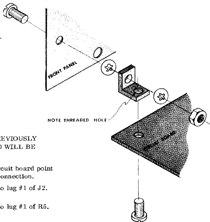
Figure 3 - Mounting Front Panel
