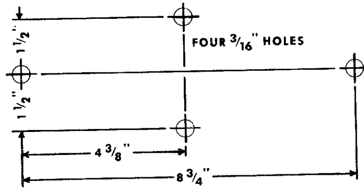
Figure 6 - Reverb Spring Mounting Hole Drilling Template
